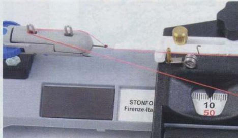
2 Put the line through the hook eye, or against the shaft (spaded)
